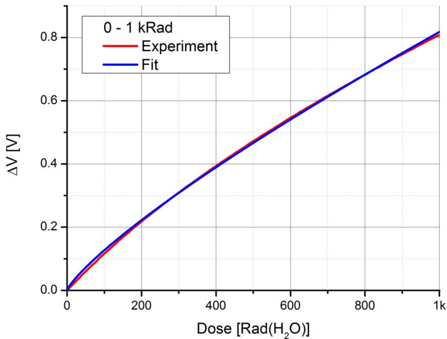
Figure 3: Typical calibration curve indicating change in voltage during irradiation. Irradiation at room temperature with Co-60 gamma source, dose rate ~30 Gy/h (3 krad/h). Voltage measurements were performed at room temperature.
