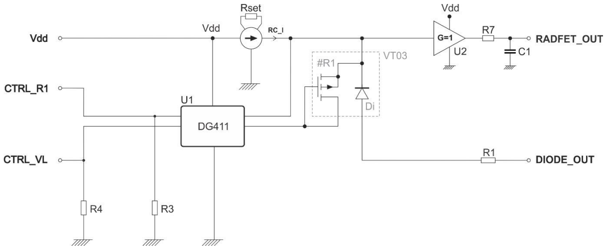
Figure 2: RM-VT03-A schematic diagram.
