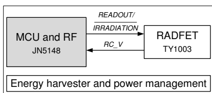
Fig. 2. Block diagram of prototyped wireless sensor node.
