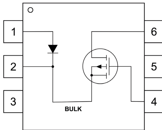
Figure 1: VT03 pin-out drawing.
