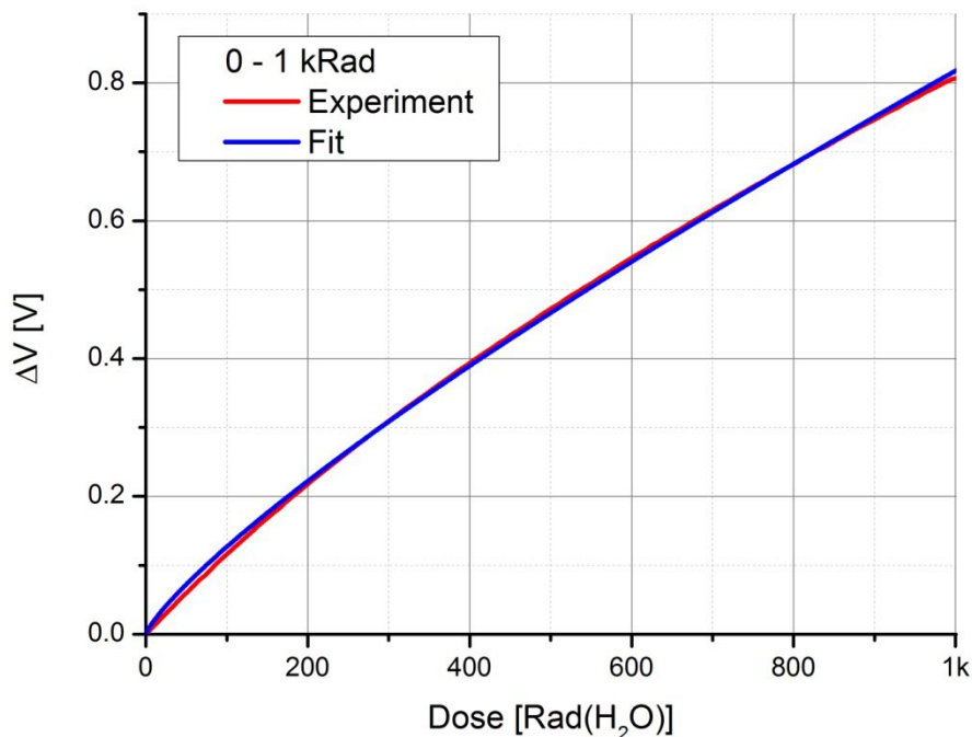
Figure 4: Typical calibration curve indicating change in RC_V during irradiation. Irradiation at room temperature with Co-60 gamma source, dose rate ~30 Gy/h (3 krad/h). All RADFET terminals grounded during irradiation. Measurements at room temperature.
