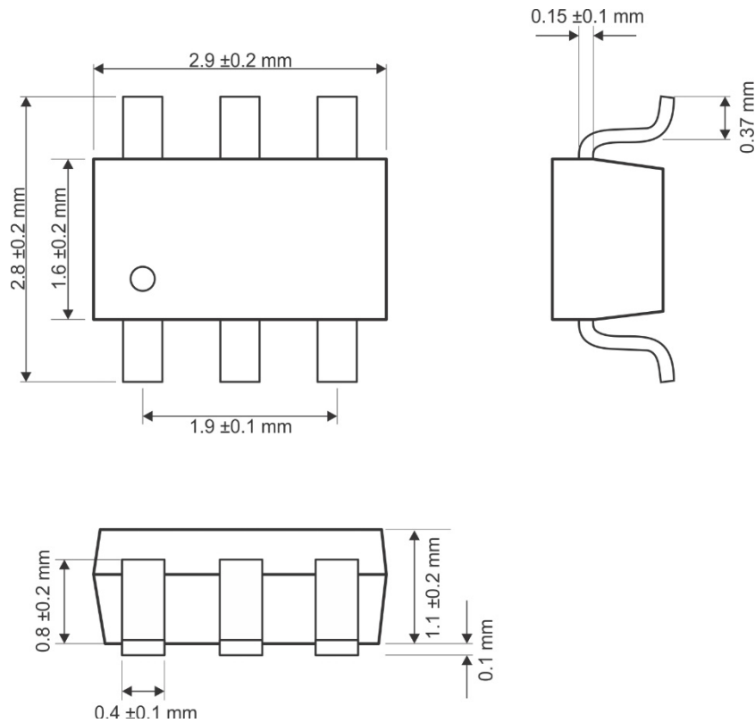
Figure 5: VT03 package diagram.
