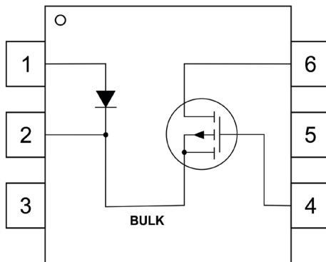
Figure 1: VT05 pin-out drawing.
